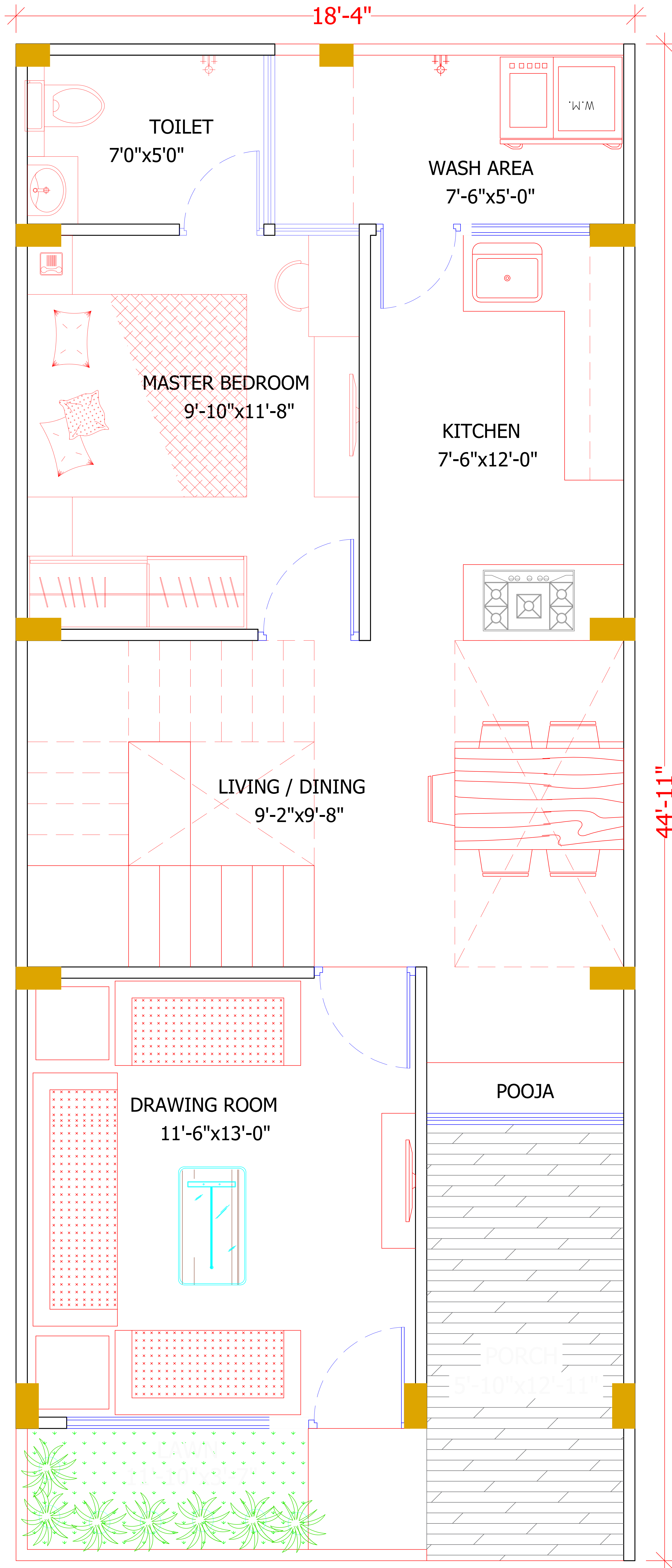
GROUND FLOOR
