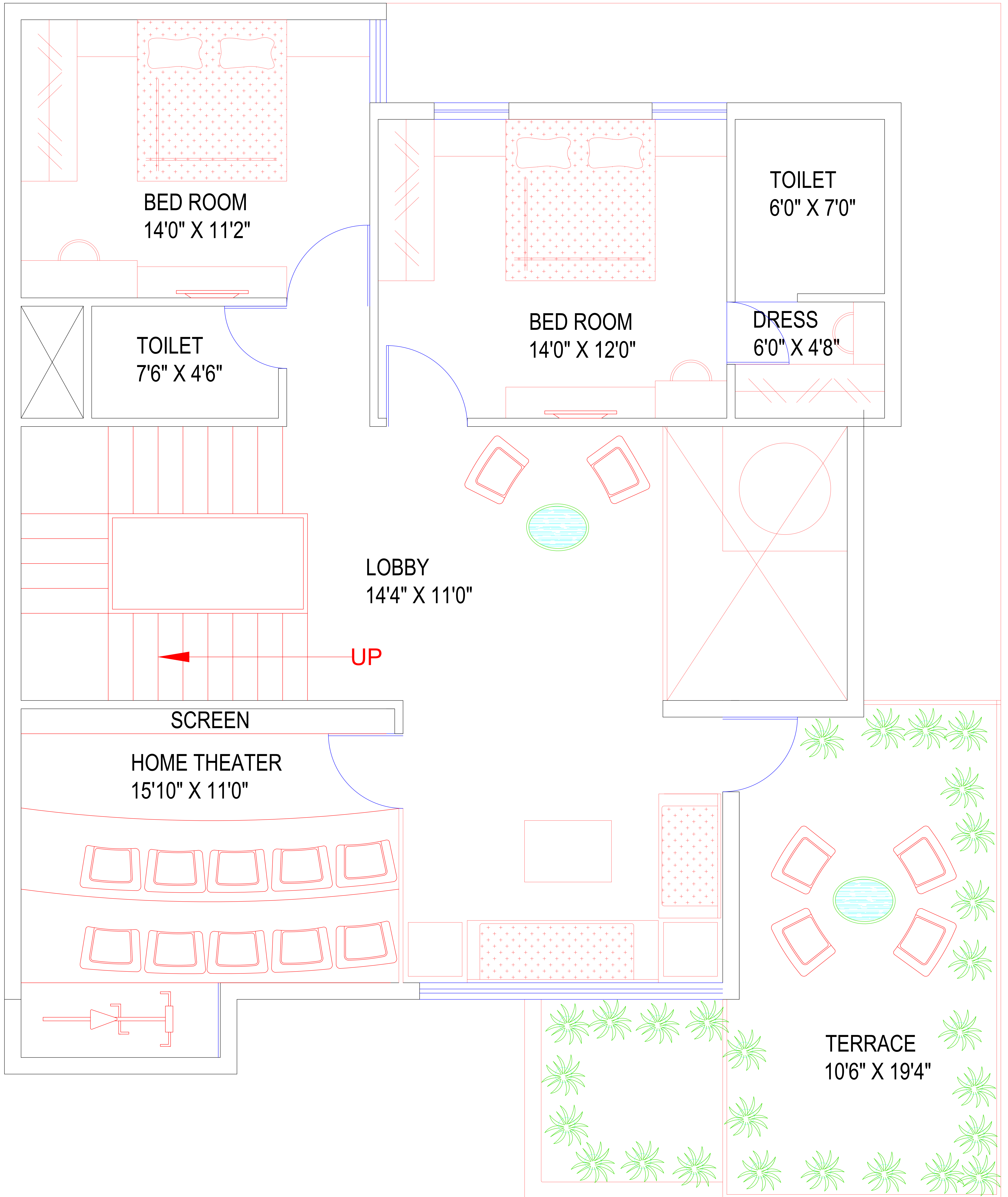
FIRST FLOOR
