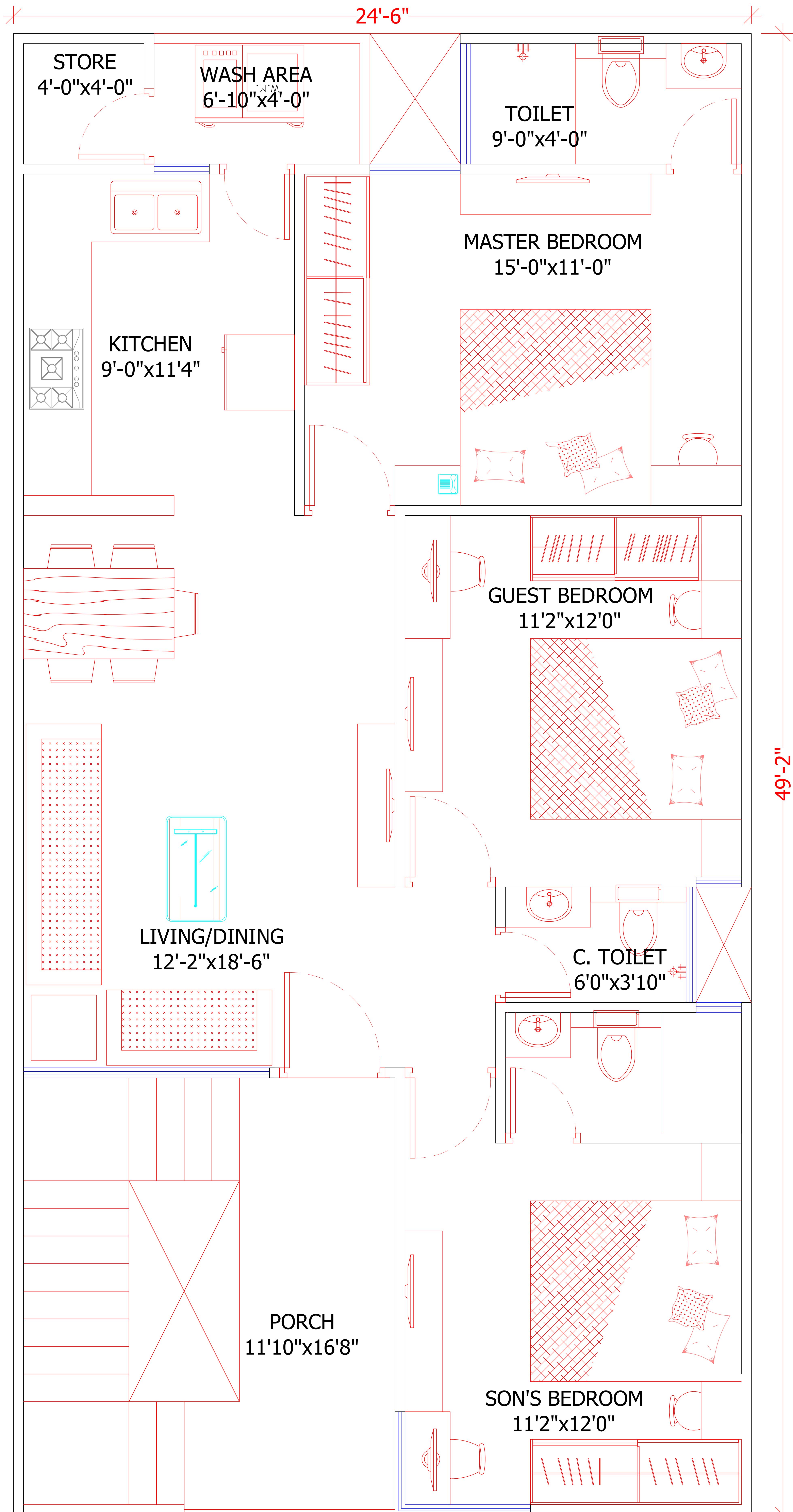
FIRST FLOOR
