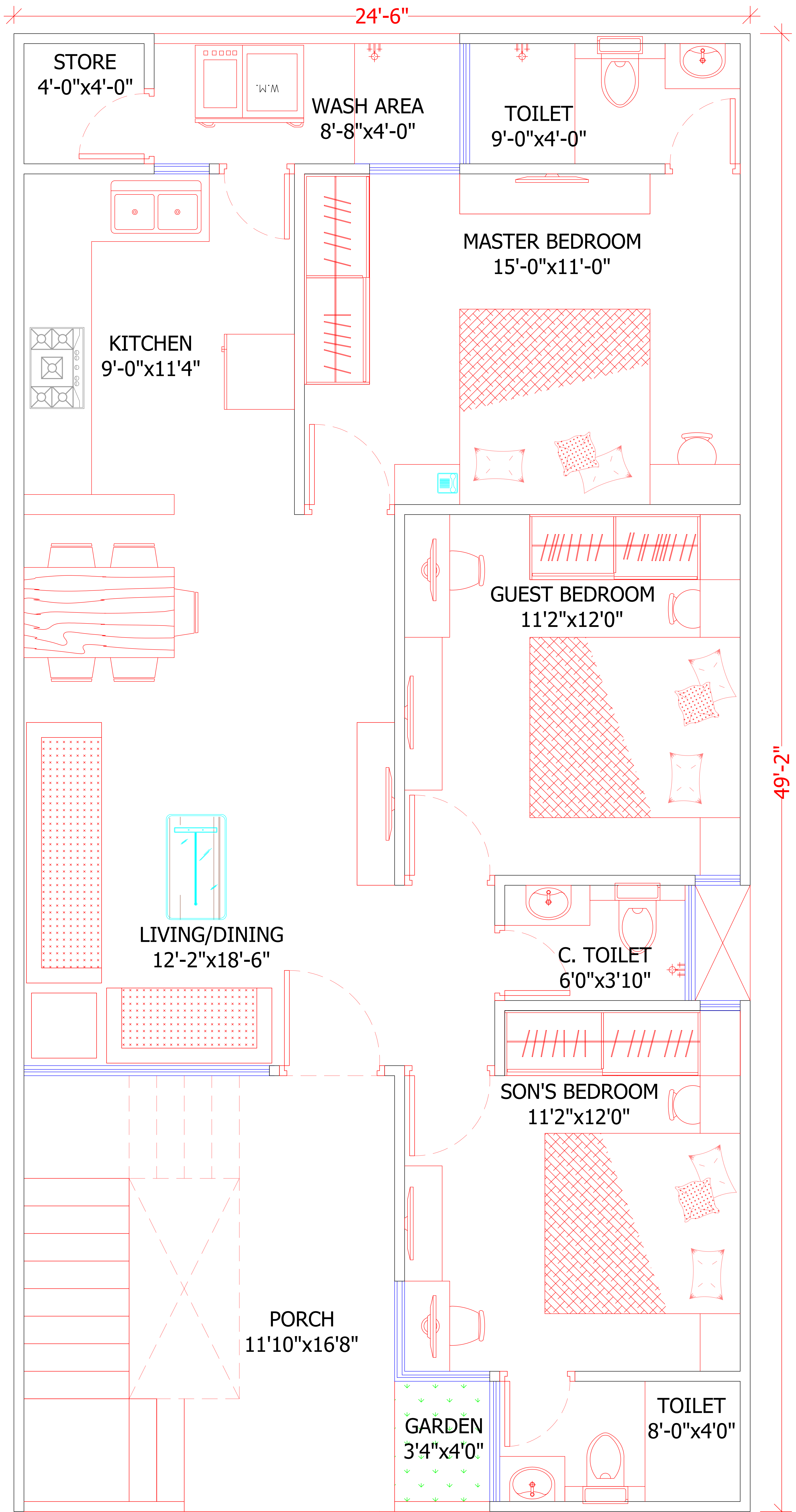
GROUND FLOOR
